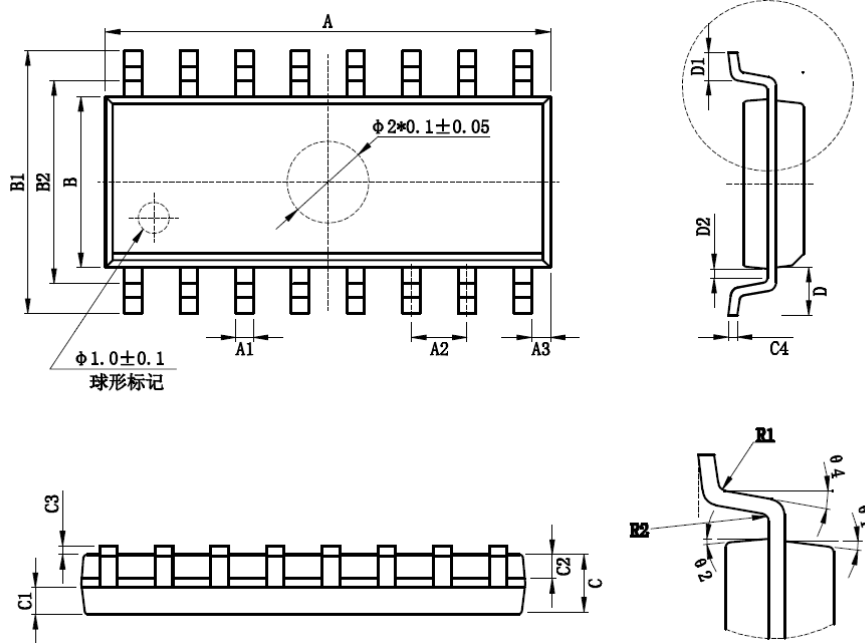
Figure 2 SOP16封装外形
